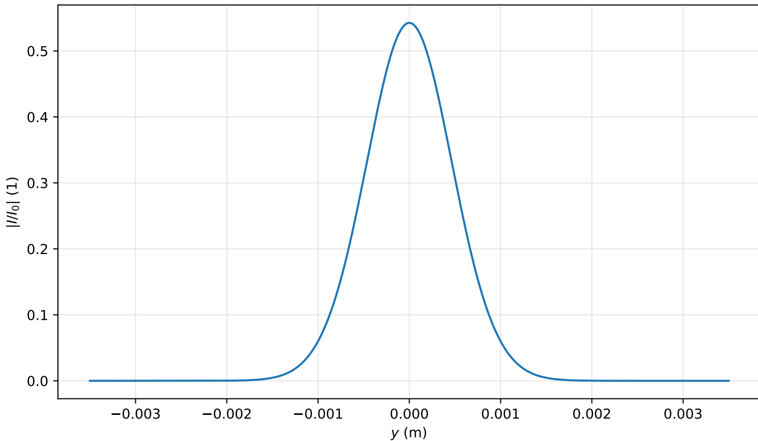
Intensity profile I(x=0, y, z=1.990)/I_0 , P_{in}=0.1P_{cr} , artificial time
